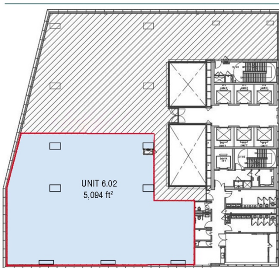
FLOOR PLAN
